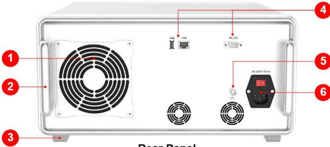
Rear Panel
